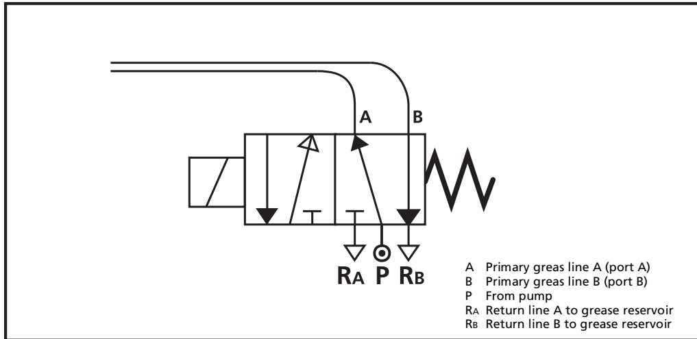
Figure 2.6 5/2-way valve
